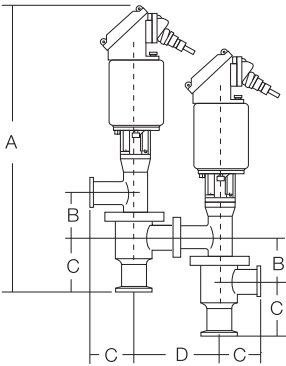
762 Individual Flo Diversion Valves
