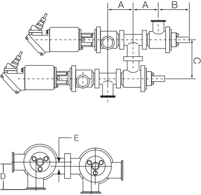
762 Reverse Acting Flo-Diversion Valve
